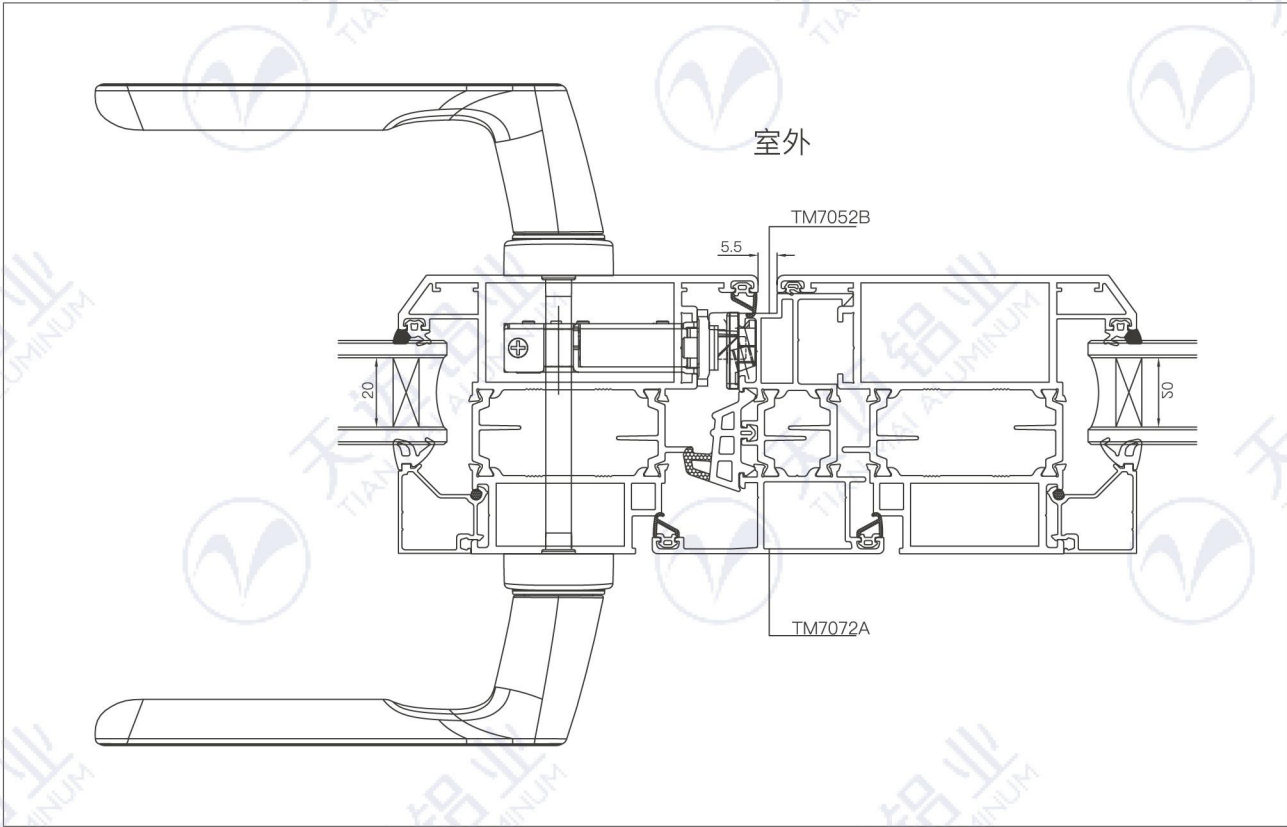
内开门对开收口装配 INWARD OPENING FRENCH DOOR TRIM ASSEMBLY
