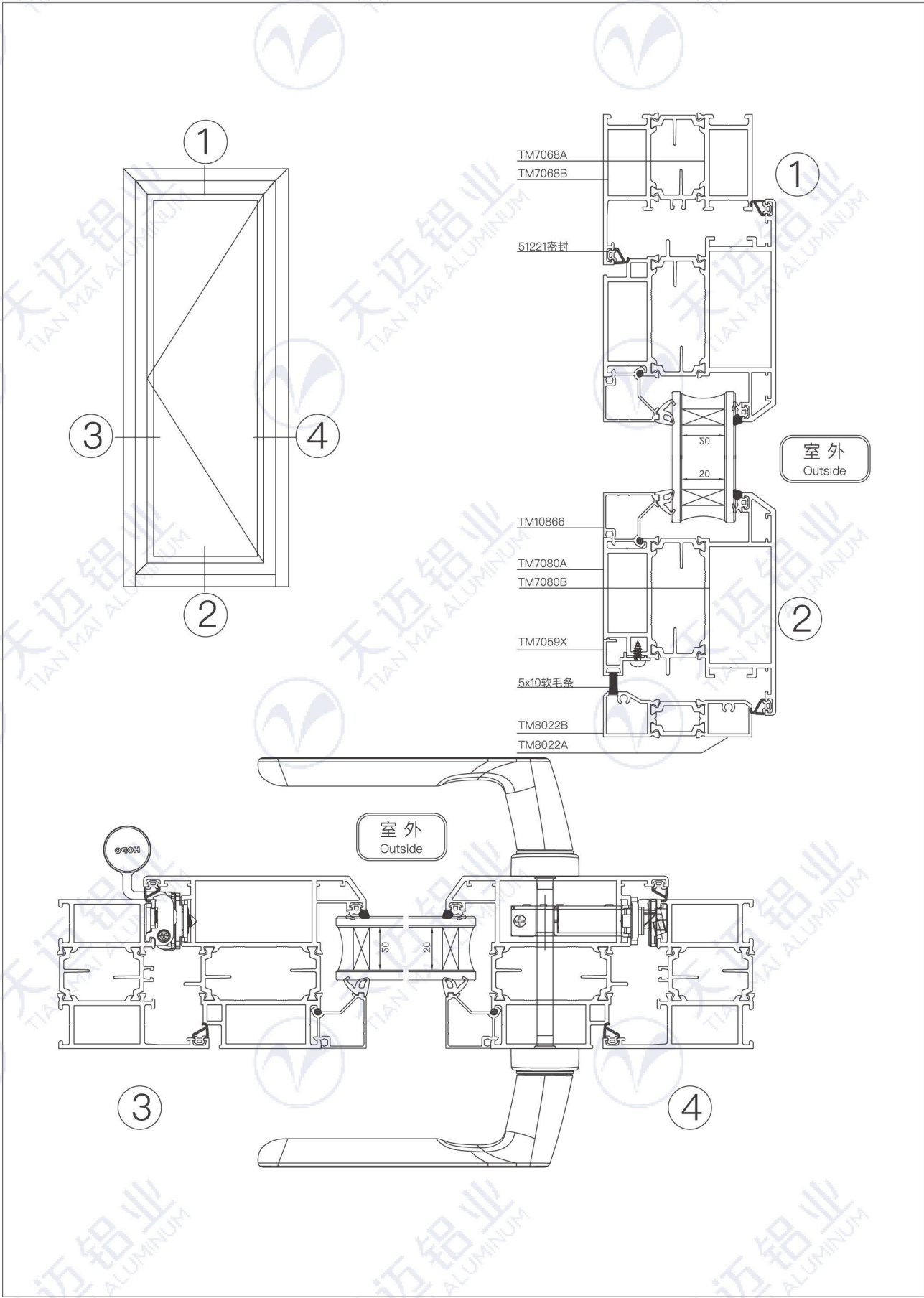
天迈平开门 70 系列断桥型材装配图 (外开平开门、不带转换) TIANMAI CASEMENT DOOR 70 SERIES THERMAL BREAK PROFILE ASSEMBLY(OUTWARD OPENING CASEMENT DOOR、NO SHIFT)
